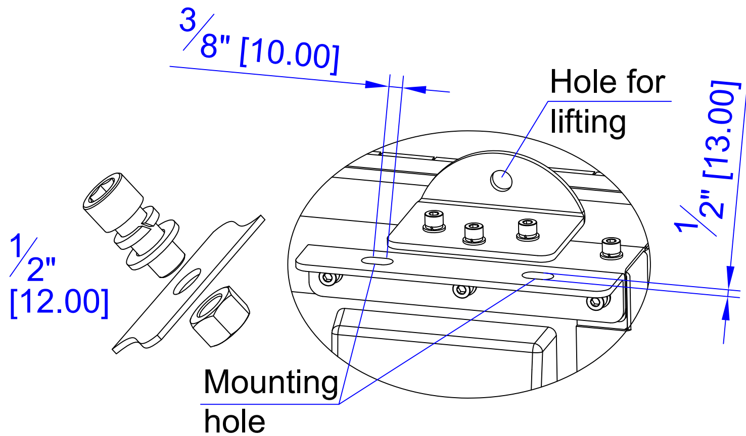
DETAIL A
