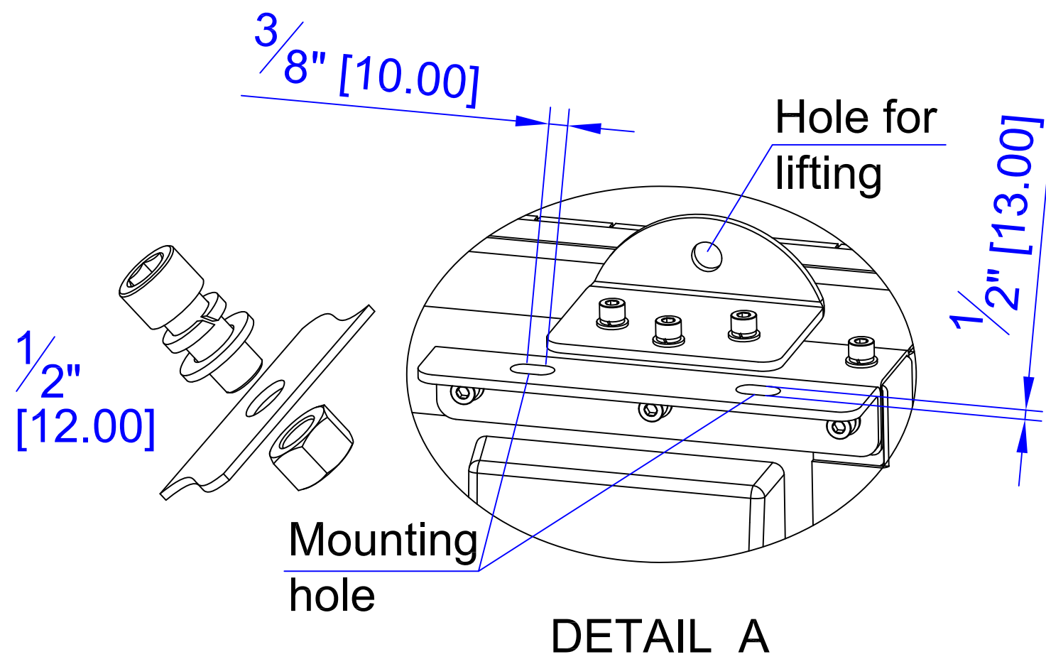
DETAIL A
