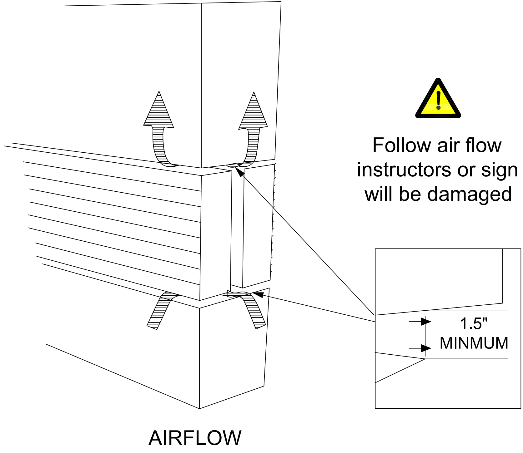
AIRFLOW
