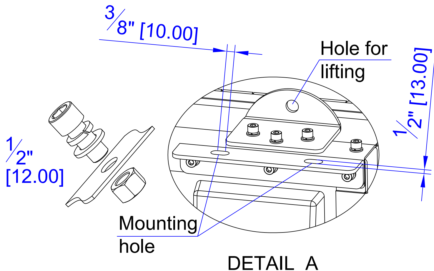
DETAIL A
