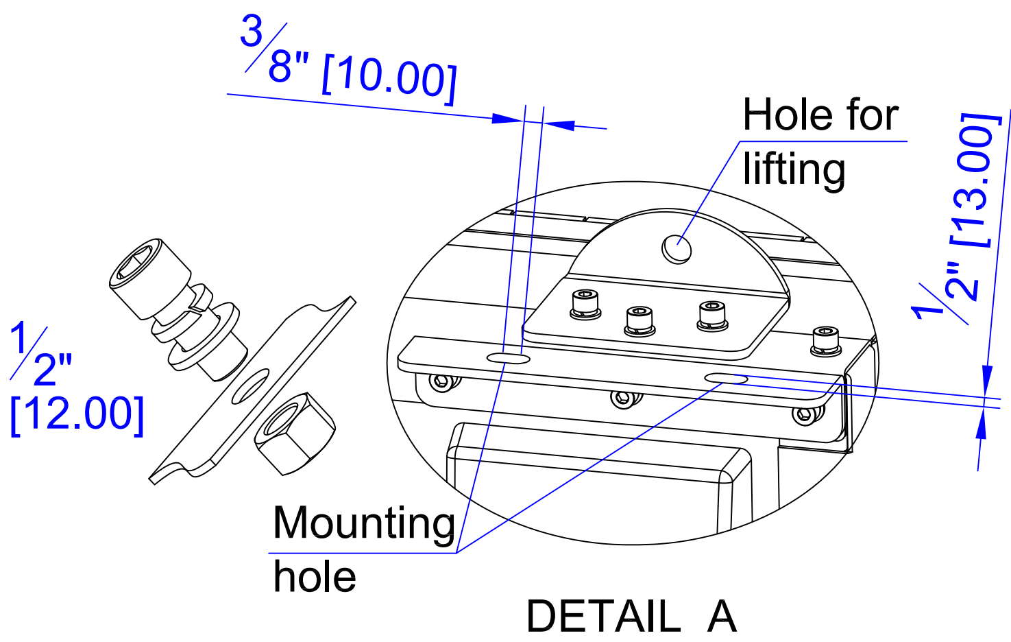
DETAIL A
