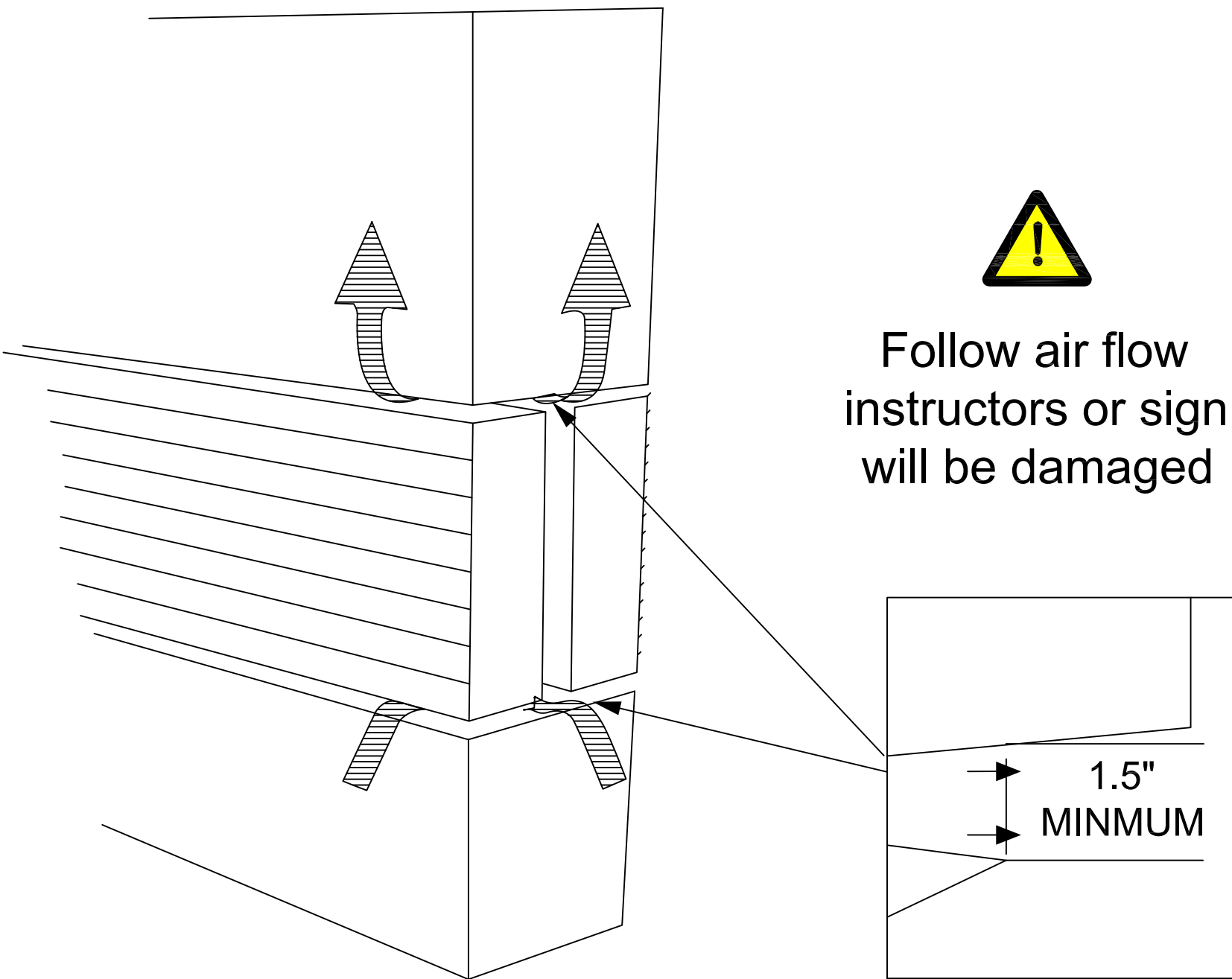
AIRFLOW
