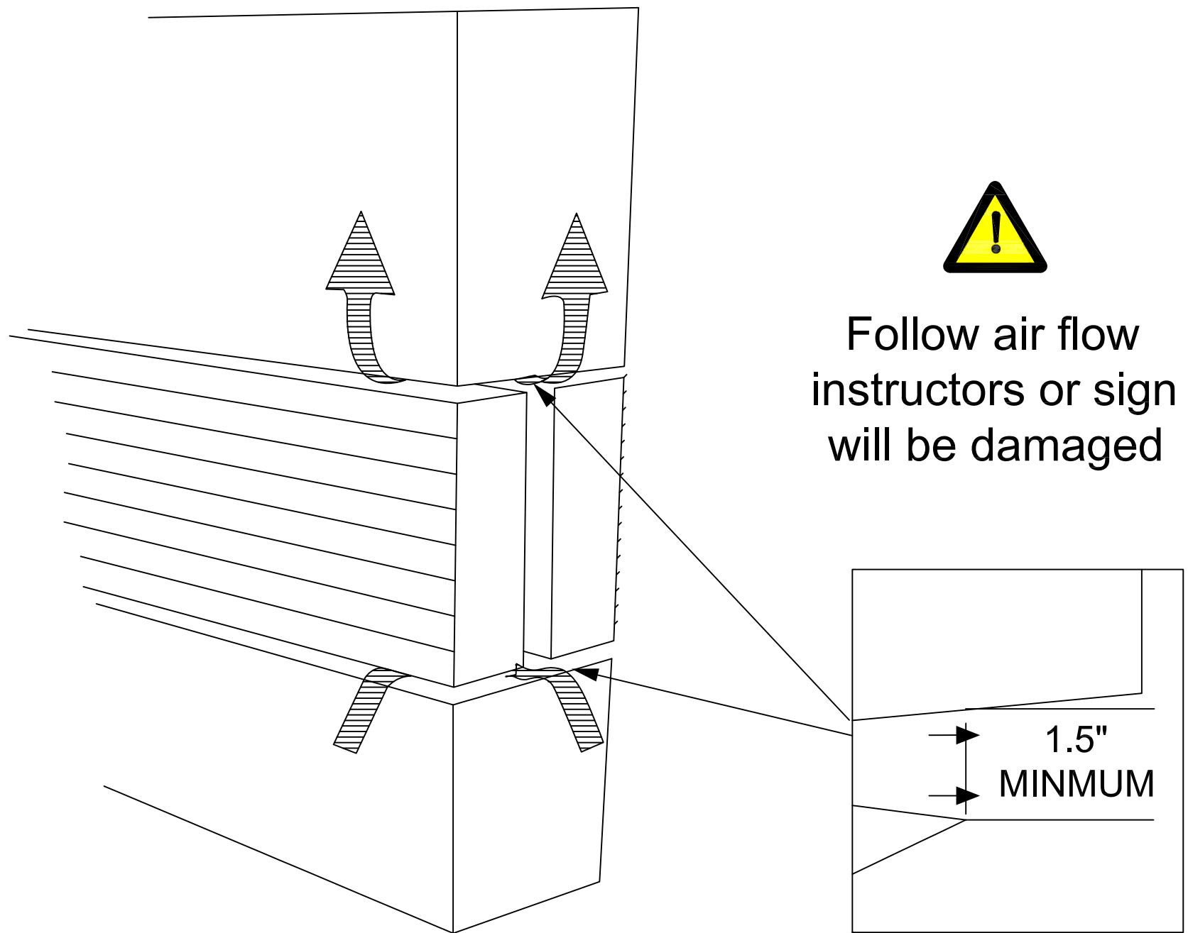
AIRFLOW
